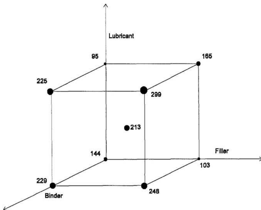
Figure 30 A cube representation of a factorial design
