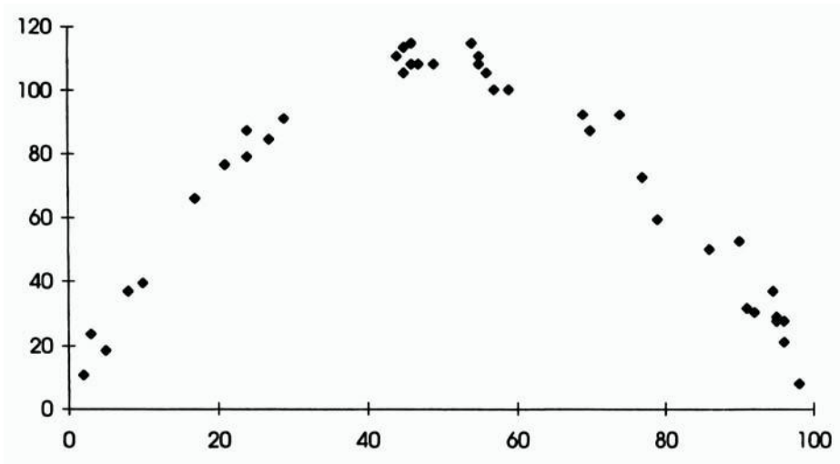
Figure 27 Precipitation vs. antibody concentration
