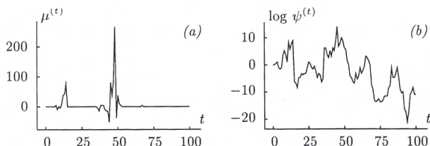
Figure 4.5. First 100 iterates of (a) \mu and (b) \log \psi from a single run of data augmentation with a nonexistent posterior.
