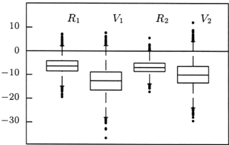
Figure 9.5. Boxplots of simulated regression coefficients from 5000 iterations of DABIPF under the alternative model.
