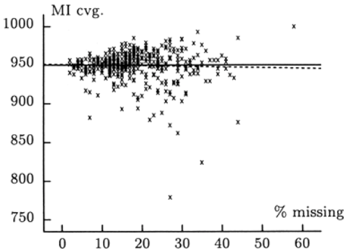
Figure 9.6. Simulated coverage of 95% multiple-imputation (MI) intervals by average percent missing information for 448 means.
