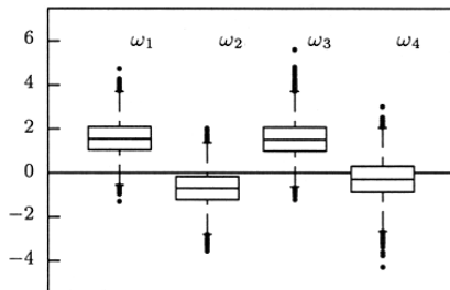
Figure 9.4. Boxplots of simulated log-odds ratios from 5000 iterations of DABIPF under the alternative model.
