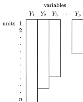
Figure 6.8. Monotone missingness pattern.
