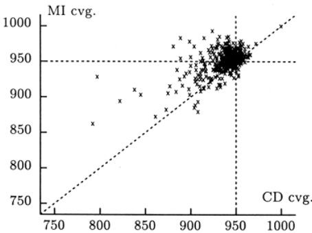
Figure 9.7. Simulated coverage of 95% multiple-imputation (MI) intervals versus complete data (CD) intervals, with points (507,824), (608, 799) and (479, 876) not shown.
