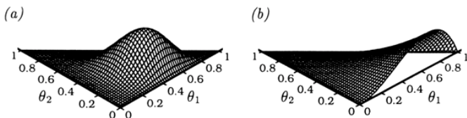
Figure 7.1. Dirichlet densities for (a) \alpha = (5, 3, 4) and (b) \alpha = (3, 1, 2) , plotted as functions of \theta_1 and \theta_2 .
