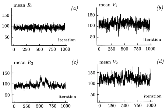
Figure 9.3. Time-series plots of the conditional means of R_1 , V_1 , R_2 and V_2 given ( G=2 , D_1=2 , D_2=1 ) for 1000 iterations of DABIPF under the alternative model.
