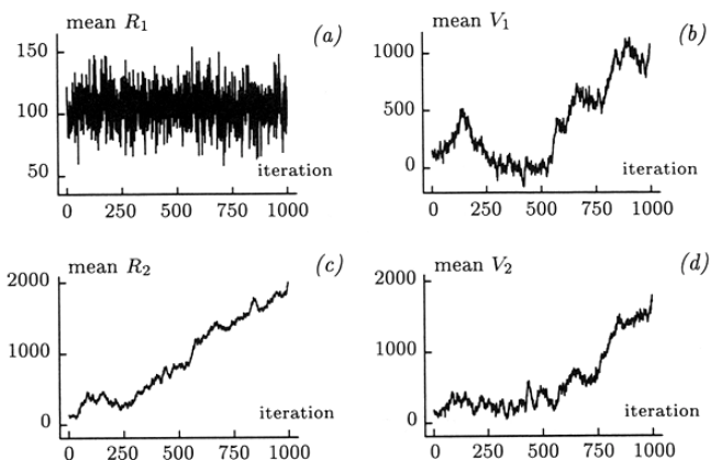
Figure 9.2. Time-series plots of the conditional means of R_1 , V_1 , R_2 and V_2 given ( G=2 , D_1=2 , D_2=1 ) for 1000 iterations of data augmentation under the unrestricted general location model.
