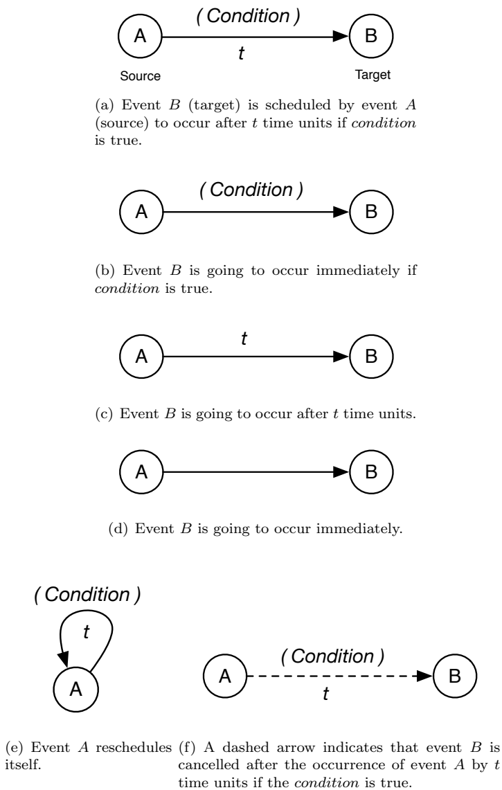
Figure 7.1 Types of edges in event graphs.
