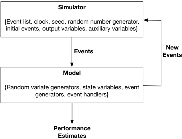
Figure 8.4 An event-driven simulation program has two independent components: simulator and model.
