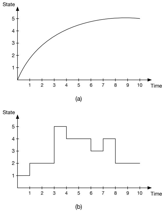
Figure 2.3 A continuous state variable takes values from a continuous set (e.g., [0, 5] in (a)). A discrete state variable, on the other hand, takes values from a discrete set (e.g., \{0, 1, 2, 3, 4, 5\} in (b)).
