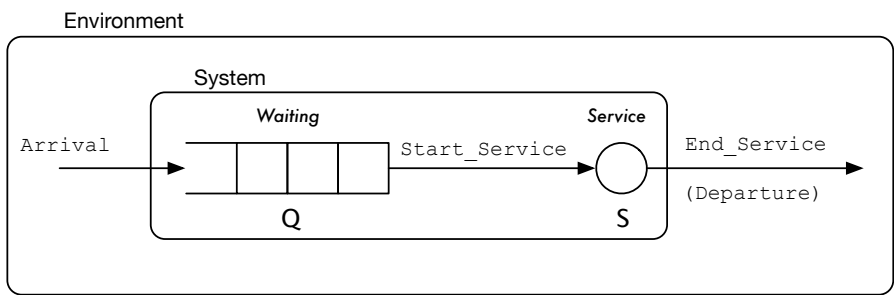
Figure 2.7 Conceptual model of the queueing situation in Figure 2.6 .
