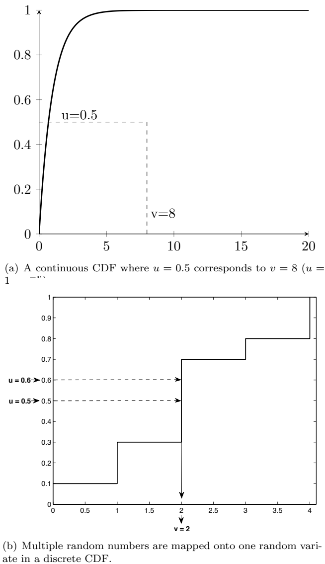
Figure 10.1 Generating random variates from cumulative distribution functions.
