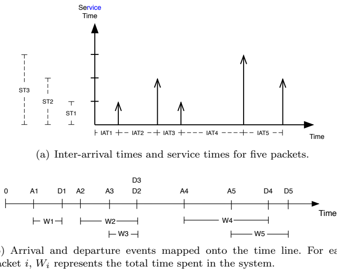
Figure 5.2 Graphical representation of the relationship between random variables and simulation events.
