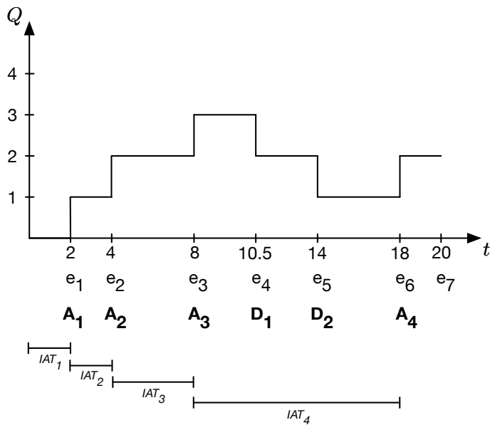
Figure 2.8 A sample path of the state variable Q which represents the number of persons in the single-server queueing system. Note the difference in the time between every two consecutive arrival events.
