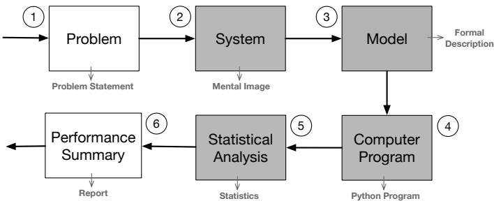
Figure 1.4 Phases of a simulation study.
