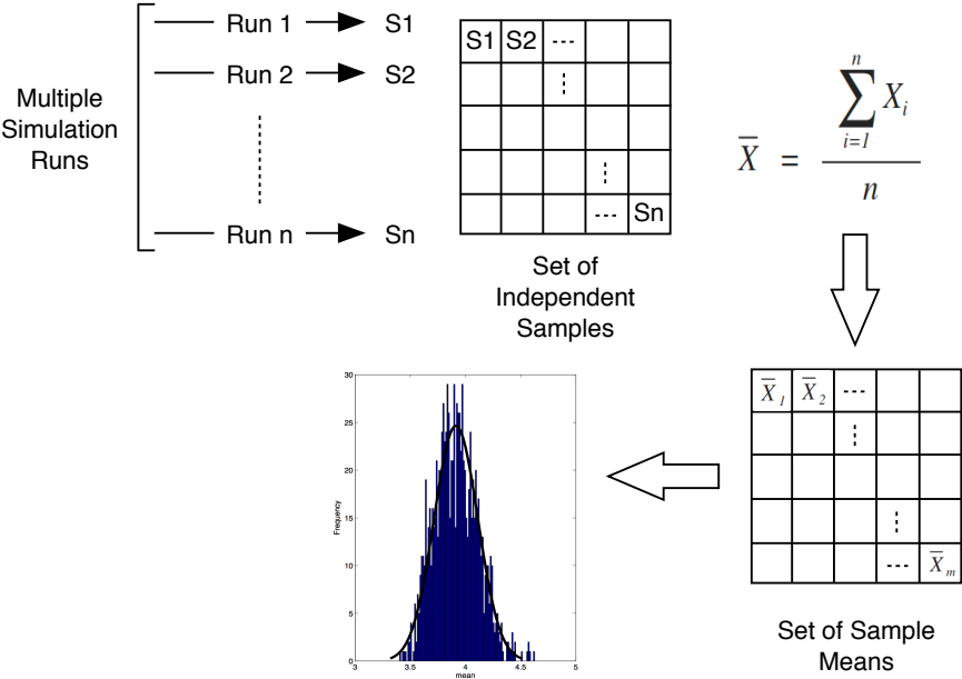
Figure 6.2 Probability distribution of the sample mean is normal.
